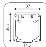
Sliding Top Track (New) BWAY-T1-1288 BM-4mtr
