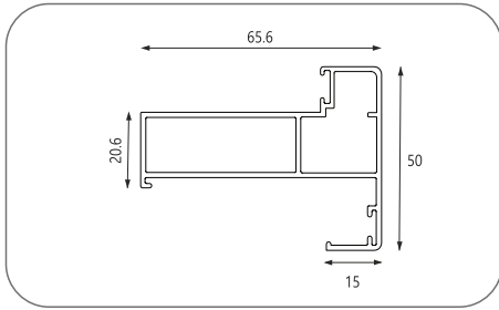
Outer Frame Profile BWAY-OFP-1350
