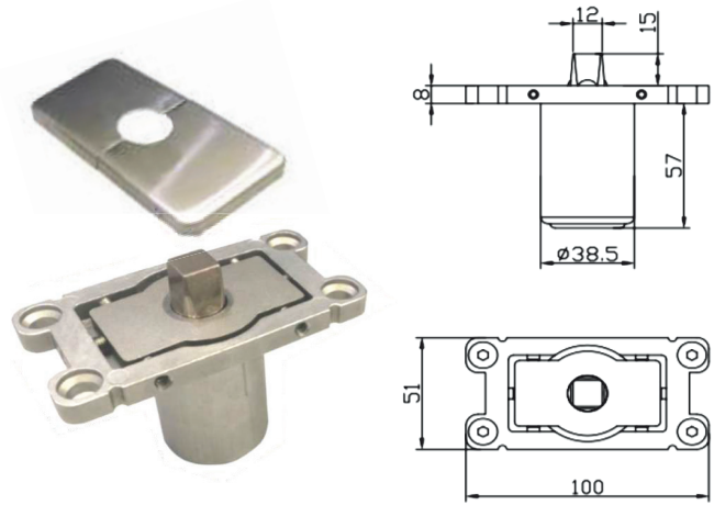
BWAY-888 - Pneumatic Floor Hinge 70kg/140kg/200kg
