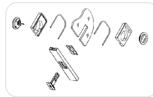
Black Matte BWAY-LOCK-01-4516-BM
