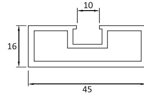
Side Profile : Code : BWAY-SP-4516
