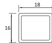
Partition Bar : Code : BWAY-PB-1618 (Georgian Bar)
