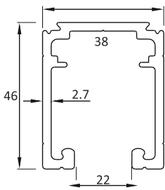
Top Track BWAY-T1
