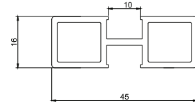
Divider Profile : Code : BWAY-DP-4517
