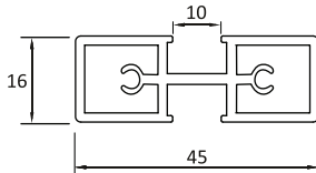
Divider Profile : Code : BWAY-DP-4516
