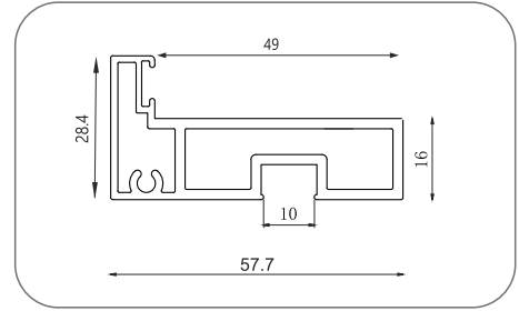
Slim Outer Frame Profile BWAY-OFP-1351
