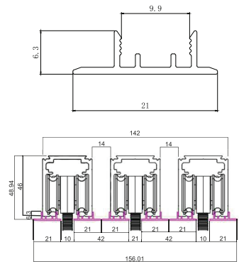
Track Concealer with Clip on : BWAY-1411 (Optional)
